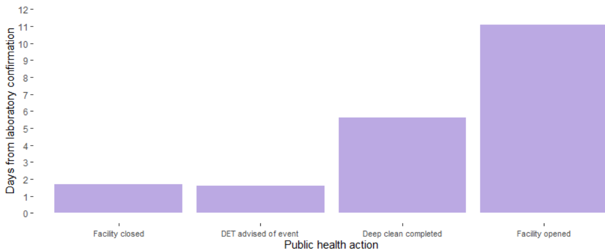
Figure 34. Days between confirmation of the first case in staff or student and school closing, DET was notified that case attended while infectious, recording a deep clean, and re-opening.
