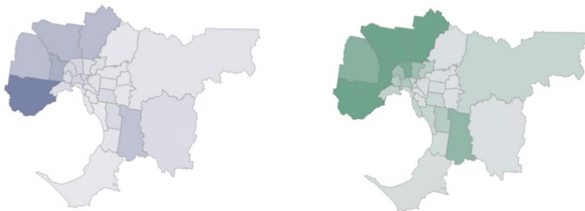
Figure 3. Geographic distribution of SARS-CoV-2 infections associated with events in ECEC and schools (left), and not associated with ECEC and schools (right). Density of shading represents number of cases in the LGA, darker shading = more cases
