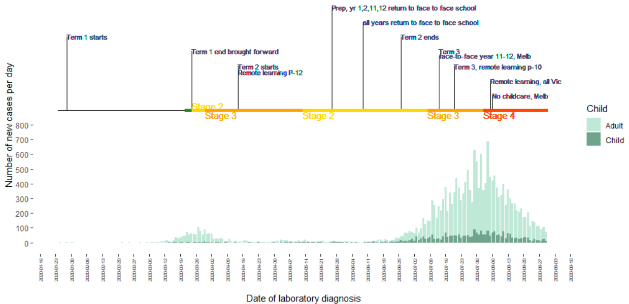
Figure 11. Victorian epidemiology curve with dates of restrictions related to ECEC and school attendance, January - August 2020.
